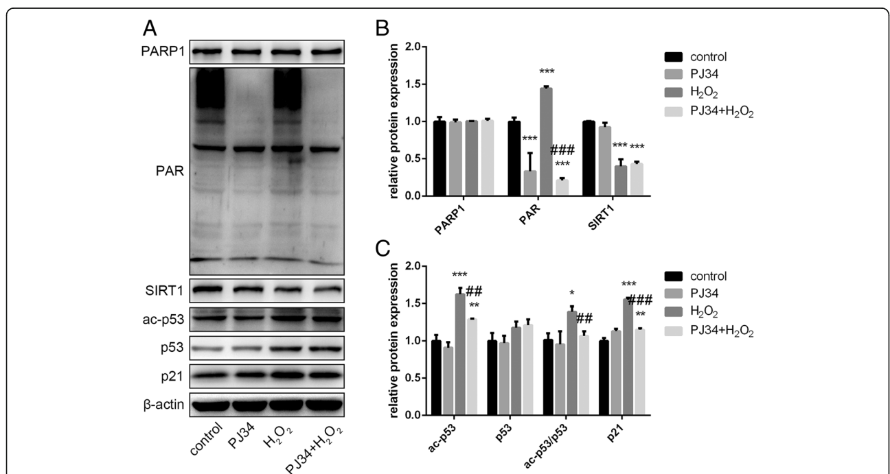
Fig. 4 Protein expression changes in senescent EPCs with PJ34 treatment. a–c Poly (ADP-ribose) polymerase 1 (PARP1), poly ADP-ribose (PAR), sirtuin 1 (SIRT1), acetylated (ac)-p53, p53, and p21 were detected by Western blot after 24 h of treatment. * P < 0.05, ** P < 0.01, *** P < 0.001, versus the control; # P < 0.05, ## P < 0.01, ### P < 0.001, versus H 2 O 2 treatment
